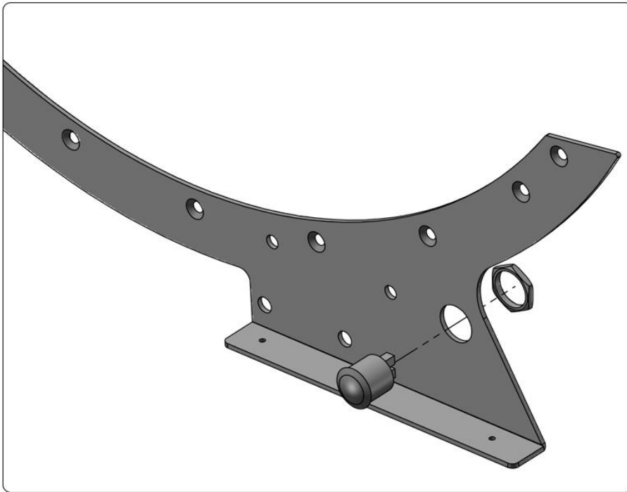
1.将开关按钮安装到机箱支架上
